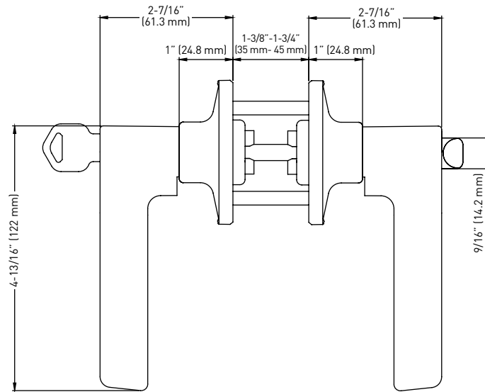
4-IN-1 ENTRY LATCH
